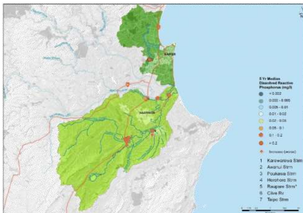
Figure 3-11: 5 year median DRP levels at Karamū and Ahuriri SoE sites. The map includes trend direction, shown with arrows. Blue arrows indicate improvement over time and red arrows deterioration. Only six years of monthly data were available for trend analysis, so caution is strongly advised with interpretation of trends.
