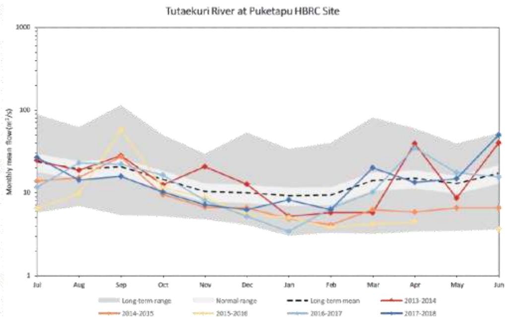
Figure 3-23: Tūtaekuri River at Puketapu HBRC Site monthly mean flow (2013-2014 to 2017-2018). Flows are shown with the long-term mean, long-term range and normal range. Note the y-axis has a logarithmic scale.
