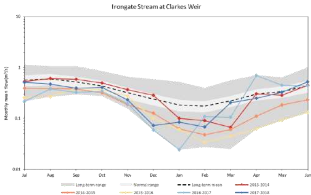
Figure 3-24: Irongate Stream at Clarkes Weir monthly mean flow (2013-2014 to 2017-2018). Flows are shown with the long-term mean, long-term range and normal range (1978-2018). Note the y-axis has a logarithmic scale.
