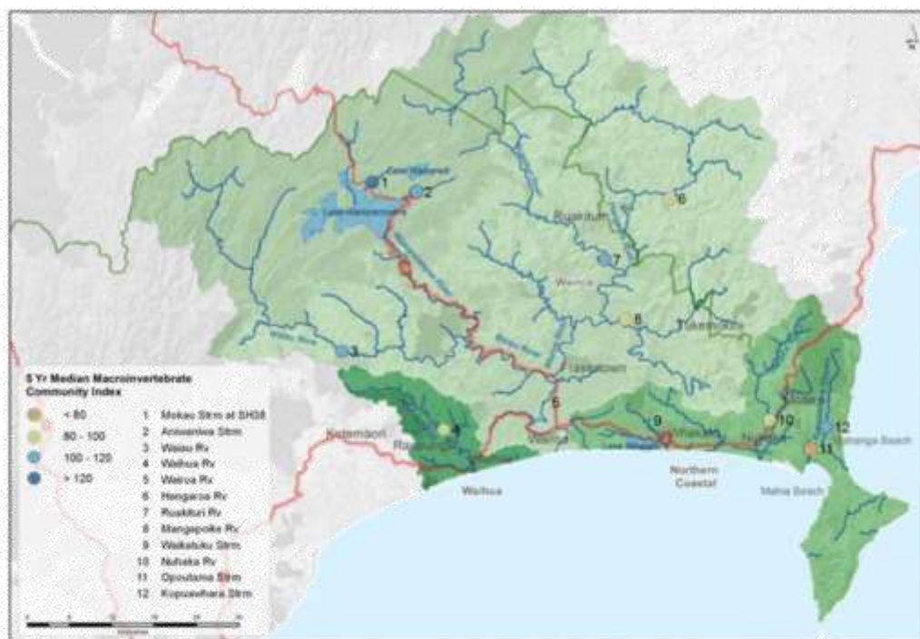
Figure 2-8: 5-year median Macroinvertebrate Community Index (MCI) observed at SoE monitoring sites of the Wairoa and nearby coastal catchments. MCI classes have been defined as: Dark blue circles – Excellent quality, clean water; Light blue circles - Good quality, possible mild pollution; Yellow circles - Fair quality, probable moderate pollution; Orange circles - Poor quality, probable severe pollution.
