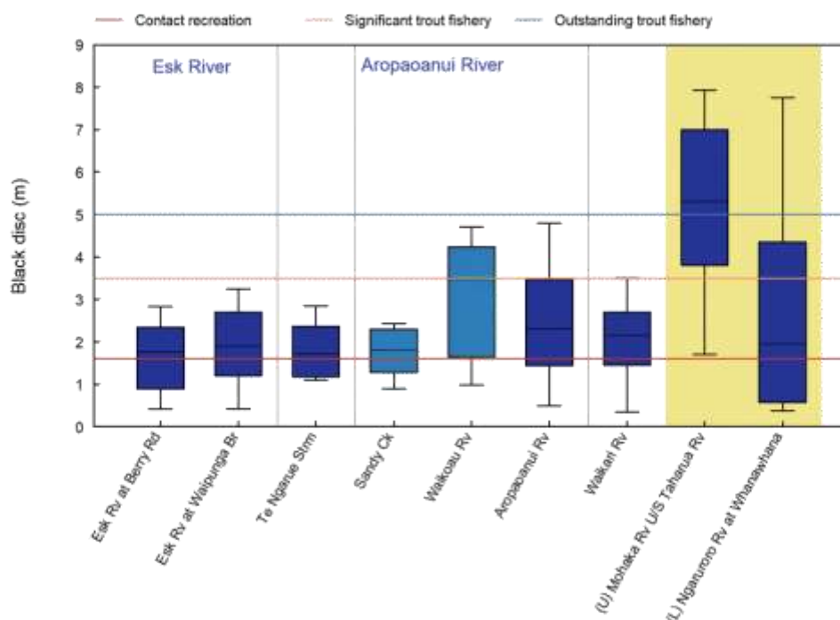
Figure 2-17: Boxplots of black disc (water clarity) for the Waikari, Esk, Te Ngarue and Aropaoanui catchments. The horizontal lines are guidelines for contact recreation and trout fisheries. Yellow shading identifies Hawke's Bay upland (U) and Lowland (L) reference sites for comparison.
