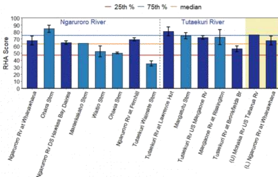
Figure 3-9: Rapid Habitat Assessment score (RHA score) at Ngaruroro and Tutaekuri SoE sites. Mainstem sites are shown with dark blue boxes, while light blue boxes are tributary sites. The horizontal lines are thresholds for physical habitat condition, with the 25th percentile = 47, median = 63, and 75th percentile = 75, of the distribution of 560 New Zealand sites. SoE sites for the Mohaka River U/S Taharua confluence and the Ngaruroro River at Whanawhāna (shaded yellow) are included as Upland (U) and Lowland (L) reference sites for comparison.
